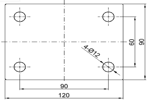
ISO 22883-2:2016, 4-view
