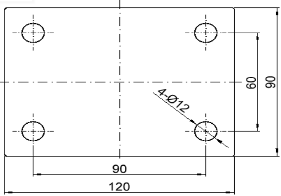
ISO 22883-2:2016, 4-view
